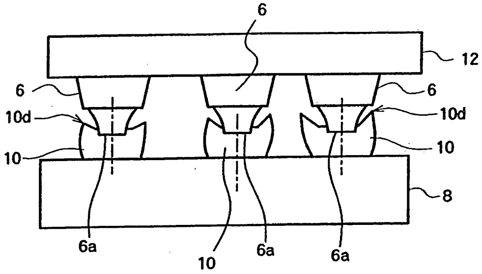
FIG. 7 PRIOR ART
